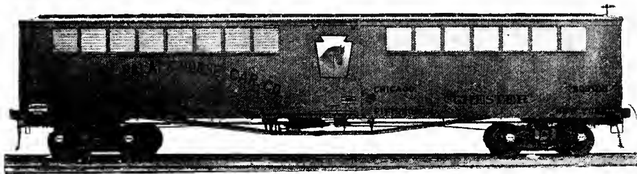
Fig. 44. STOCK CAR FOR HORSES AND PRIZE CATTLE. Equipped with Air Brakes and Swing Motion Trucks. (Interior shown in Fig. 43.)
